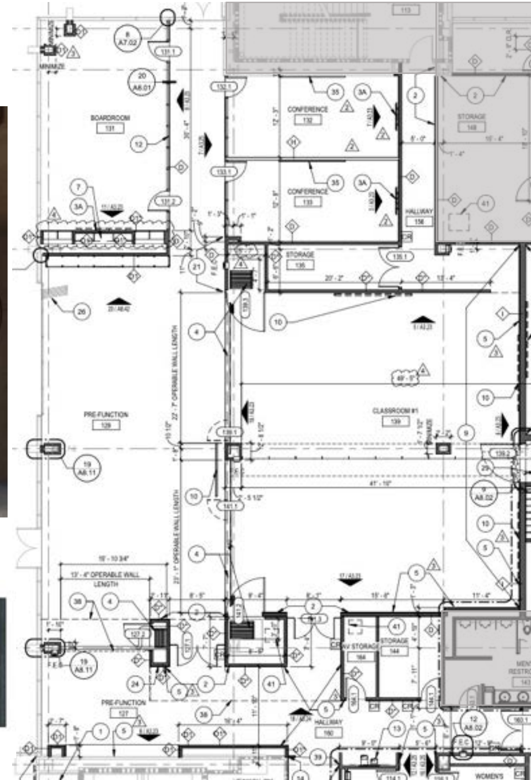
LEVEL 1 FLOOR PLAN
