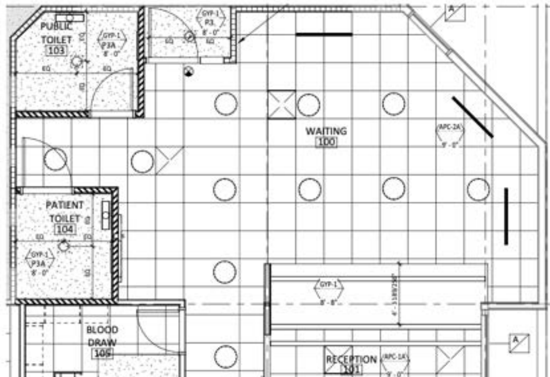
LEVEL 1 RCP
