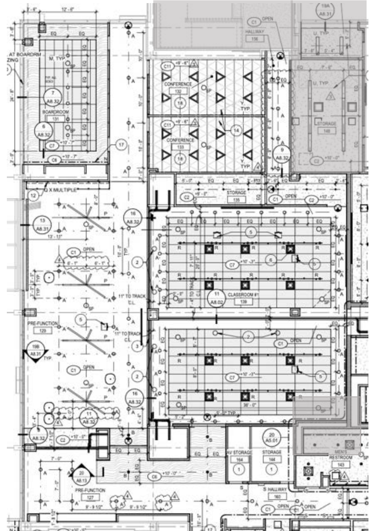
LEVEL 1 RCP
