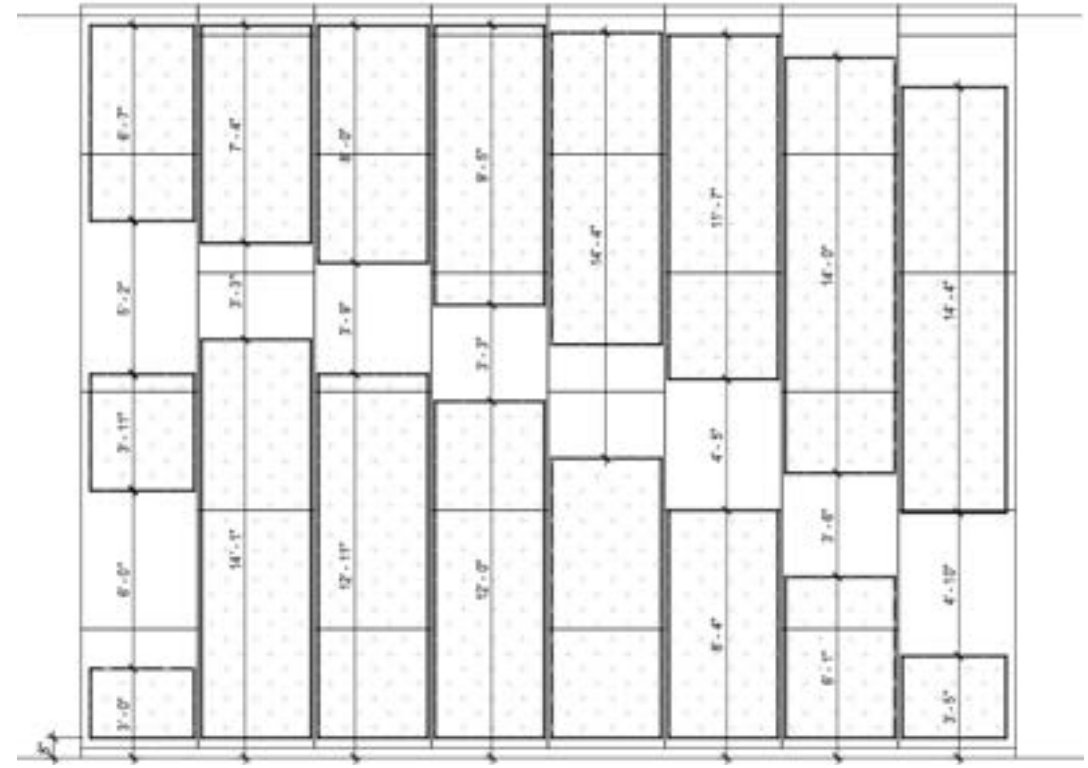
LOBBY WALL LIGHTS DIAGRAM
