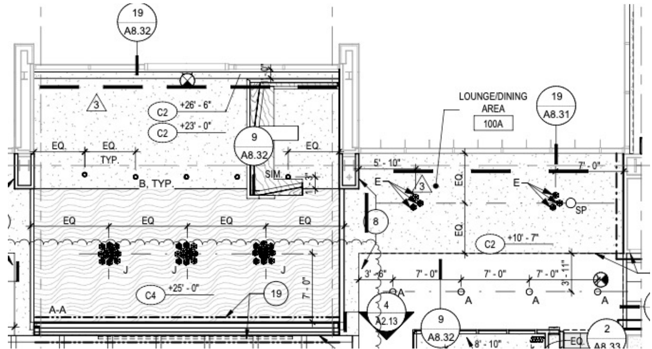
LEVEL 1 RCP
