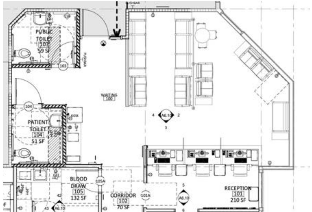
LEVEL 1 FLOORPLAN
